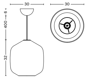
BUOY GLASS PENDANT 300 Diameter 30 cm Height 32 cm Weight 3,3 kg
