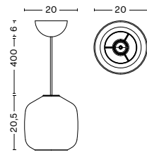
BUOY GLASS PENDANT 200 Diameter 20 cm Height 20,5 cm Weight 1,7 kg
